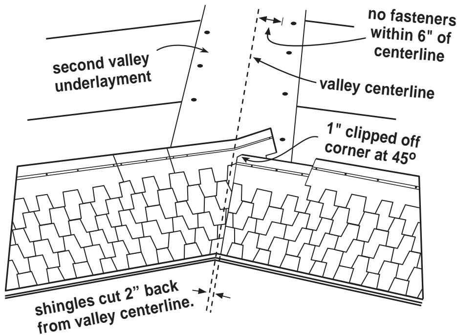
Figure 4 Closed-Cut Valley
