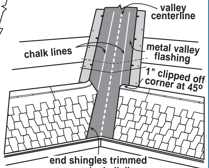
Figure 3 Shingle Application
