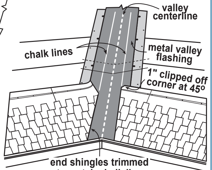
Figure 3 Shingle Application
