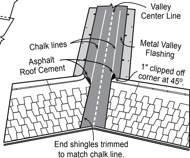
Figure 3 Shingle Application
