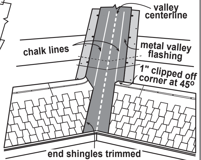
Figure 3 Shingle Application
