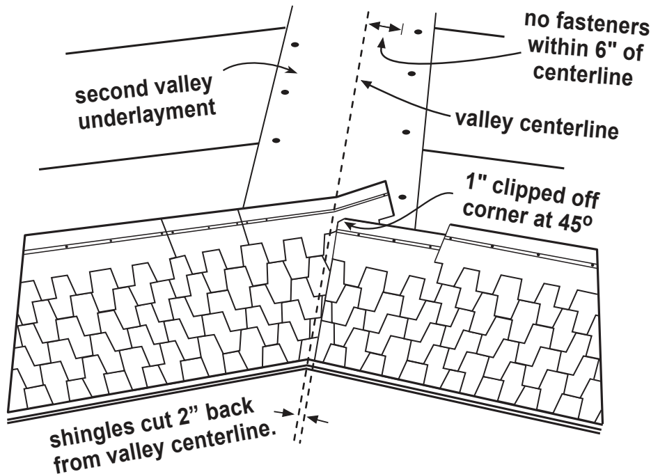
Figure 4 Closed-Cut Valley
