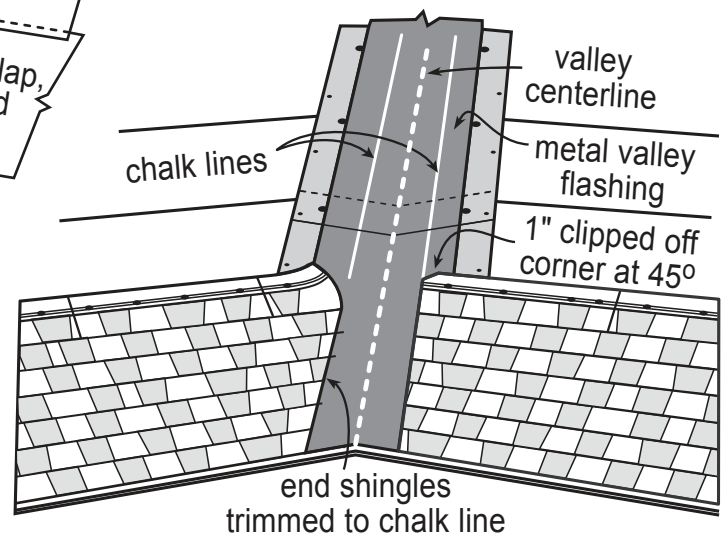
Figure 3 Shingle Application
