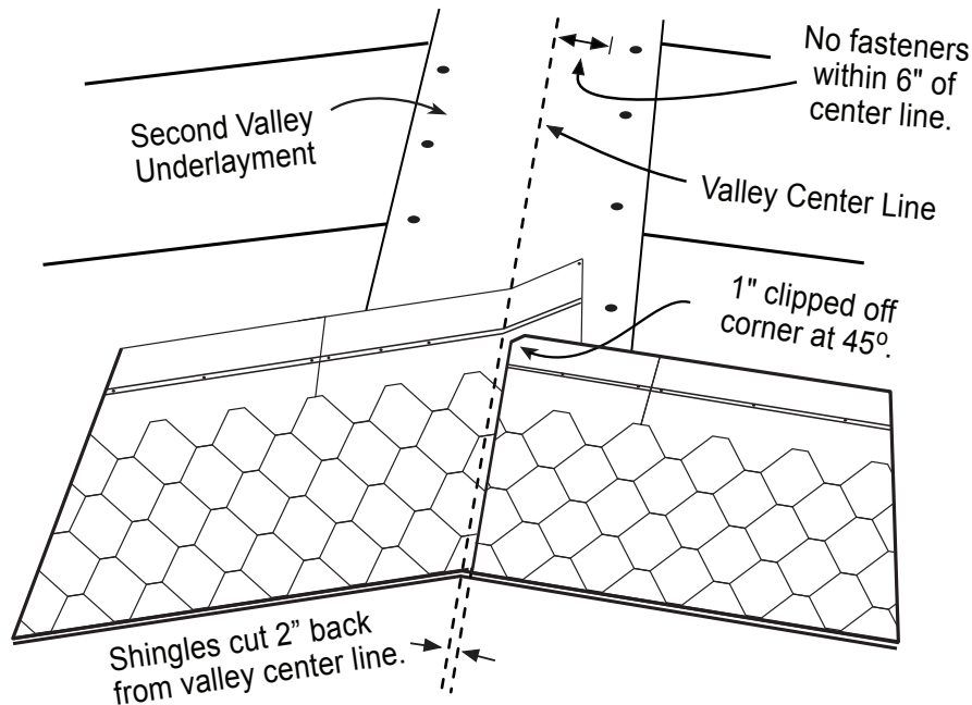
Figure 4 Closed-Cut Valley
