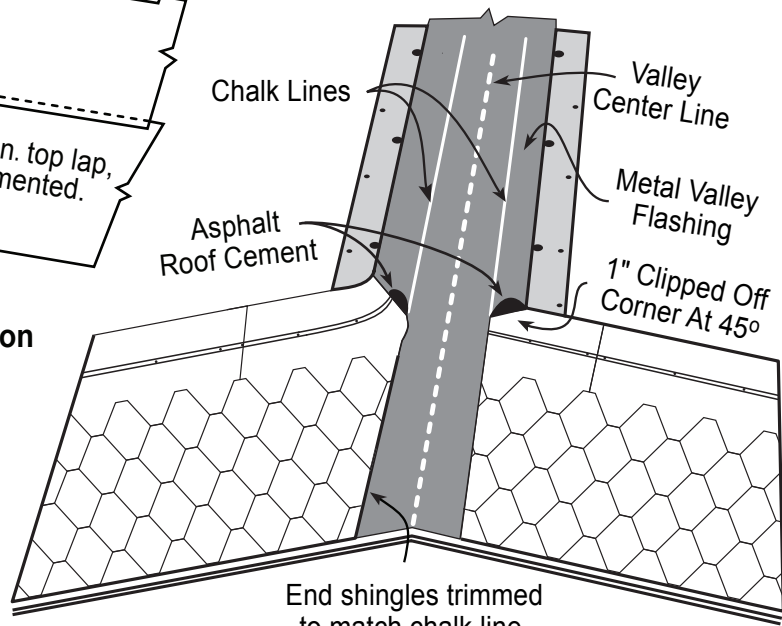
Figure 3 Shingle Application
