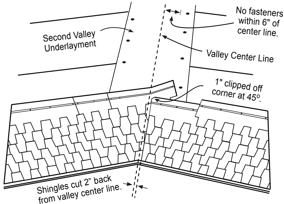
Figure 4 Closed-Cut Valley
